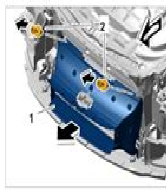
Fig. 1. Removing Front Air Guide
