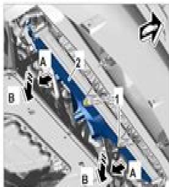
Fig. 1. Removing Lower Fastening Screws
