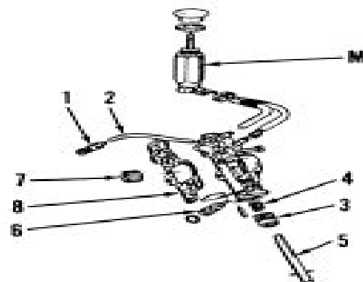
Fig. PN126—Exploded view of automatic oil pump assembly typical of all models. Model 555 is also equipped with manual pump (M).
