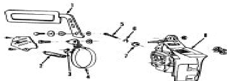
Fig. PN126—Exploded view of chain brake mechanism.
