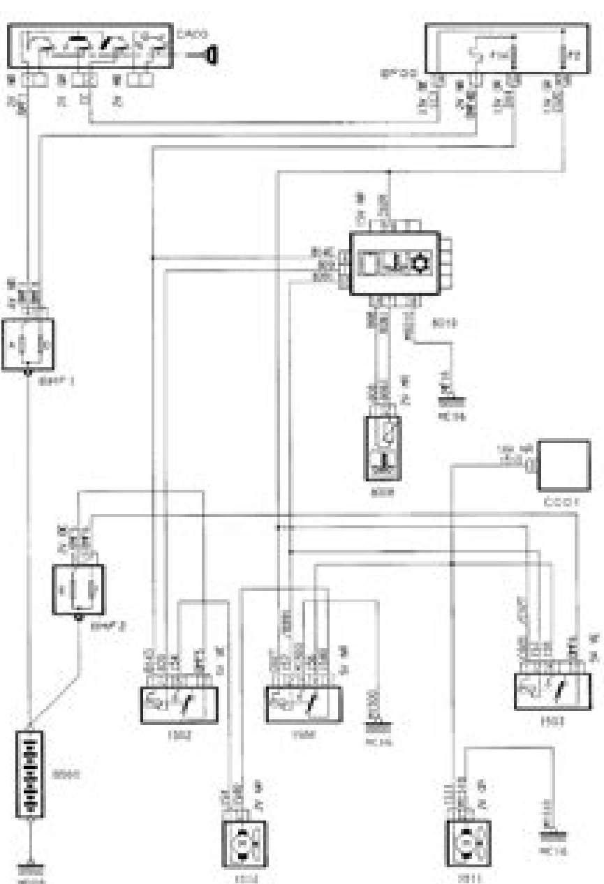
Typical diesel cooling system - models from 1998-on
