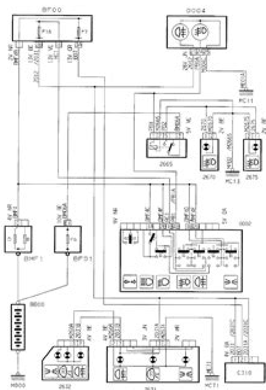
Front/rear foglights - models from 1998-on
