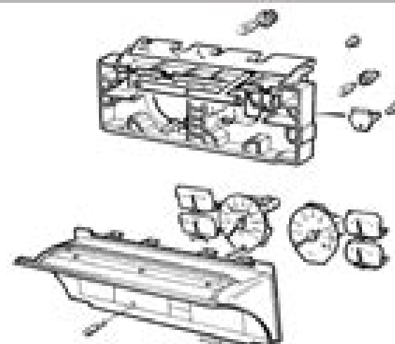
Fig. 12-9 Exploded diagram of front-right instrument panel
