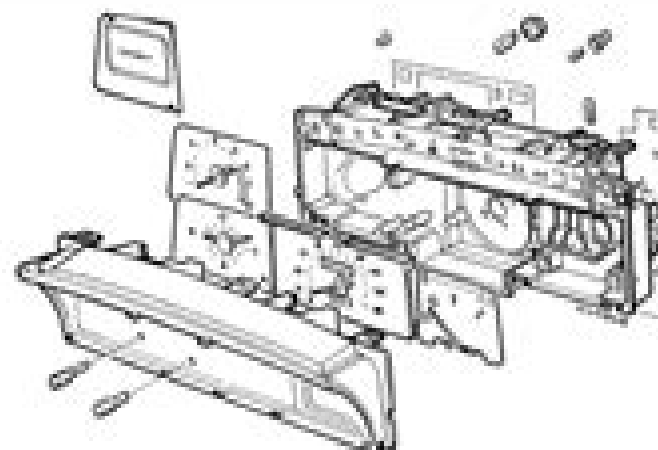
Fig. 12-8 Exploded diagram of front-left instrument panel
