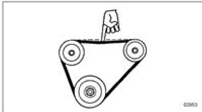
Tension Test
