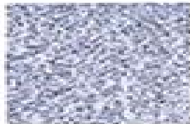
Diorite
