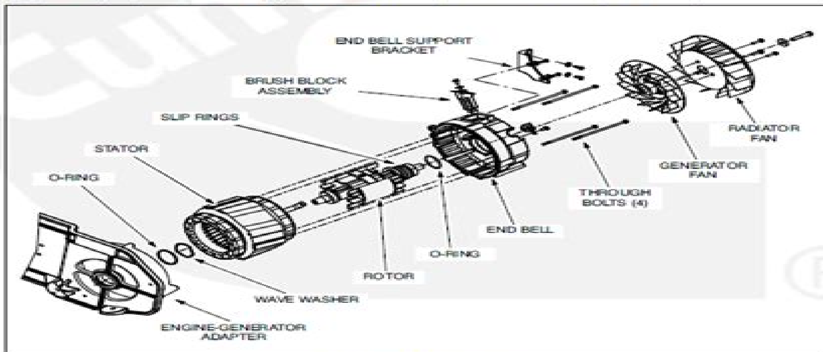
FIGURE 6-1. GENERATOR
