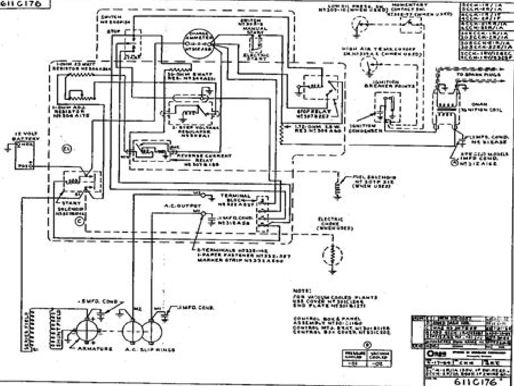
Wiring Diagram 611C176 – Remote Type Plant, Alternating Current, 120 Volt 2-Wire, and 240 Volt 2-Wire, 1-Phase
