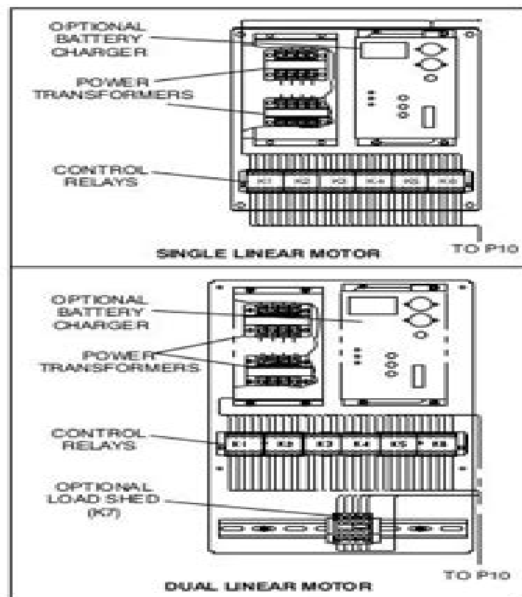
FIGURE 2-13. CONTROL PLATE
