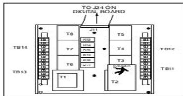
FIGURE 2-12. POWER MODULE
