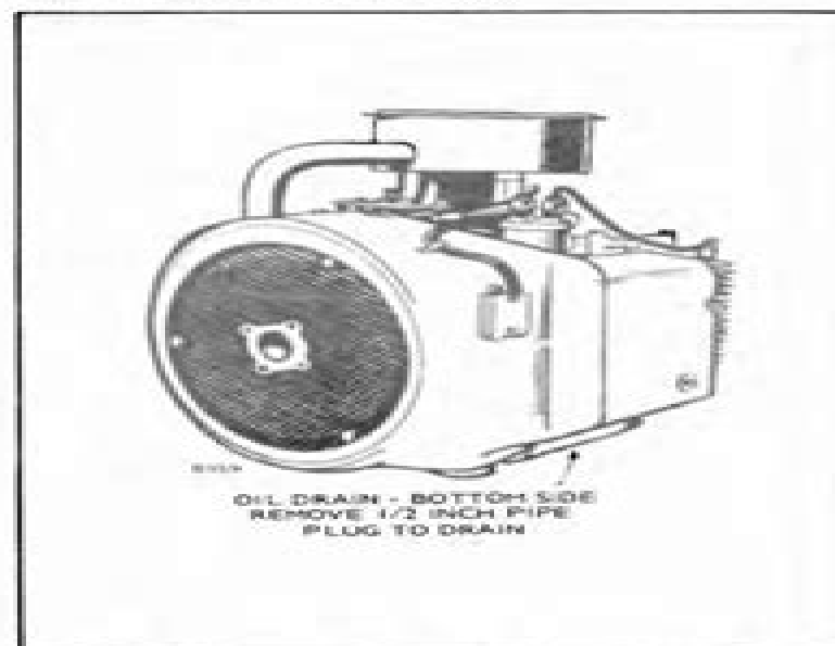
FIGURE 2. OIL DRAIN LOCATION
