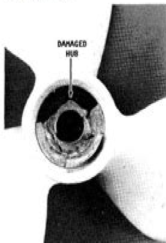
A cracked hub, caused by the propeller struck an underwater object. The rubber hub and propeller sleeve may be replaced at nominal cost.
