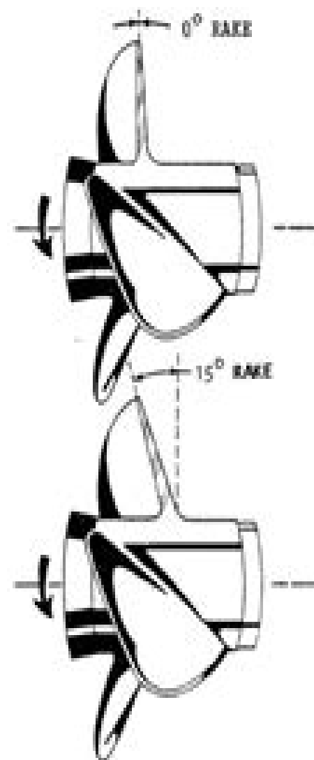
Illustration depicting the rake of a propeller, as explained in the text.
