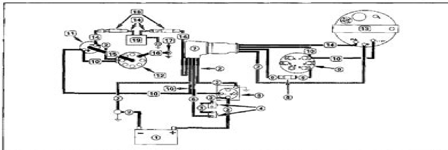
Ignition Circuit 5.7 GL and GS Models
