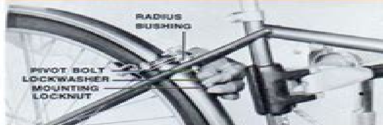
FIGURE 3—REMOVING LOCKNUT AND LOCKWASHER
