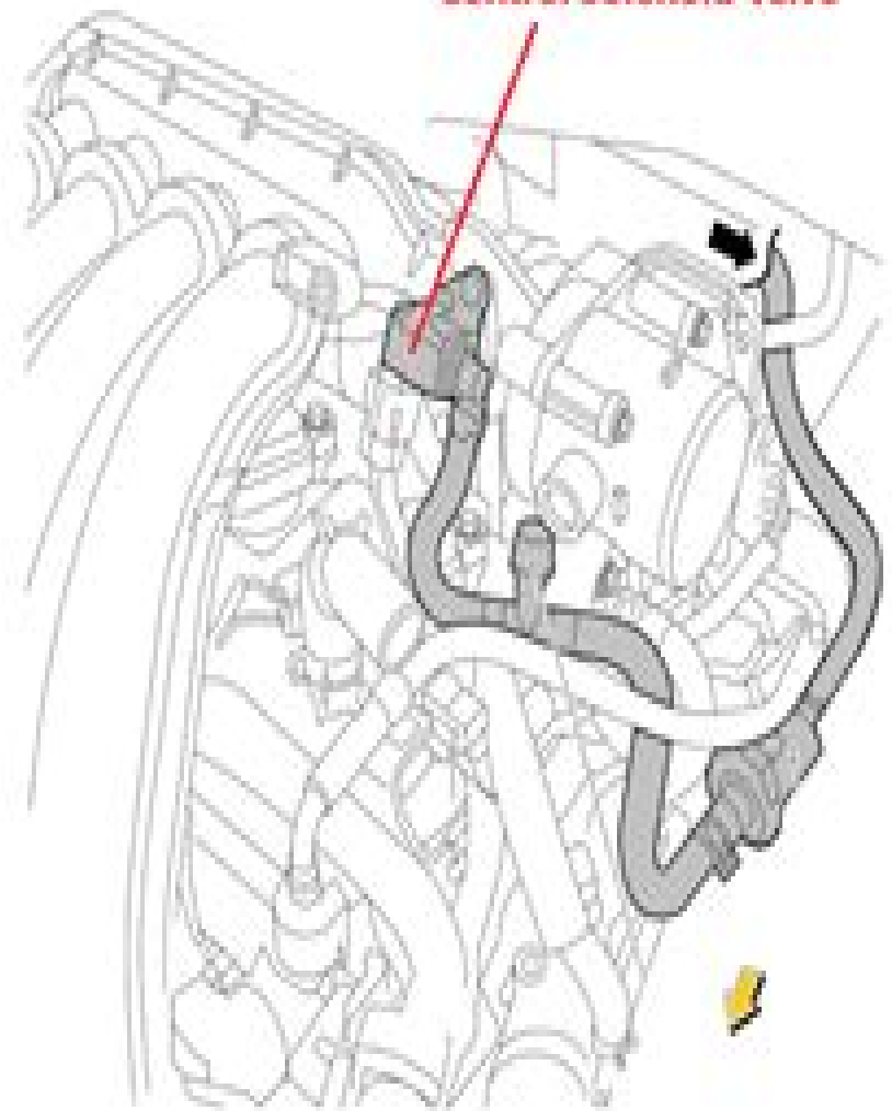
EVAP Canister Purge Volume Control Solenoid Valve
