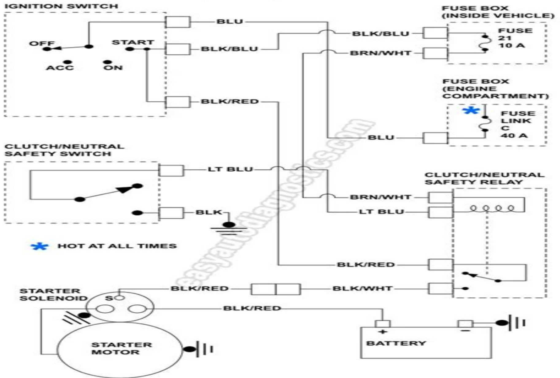
STARTER MOTOR WIRING DIAGRAM (MT) (2002-2003 3.5L MAXIMA)
