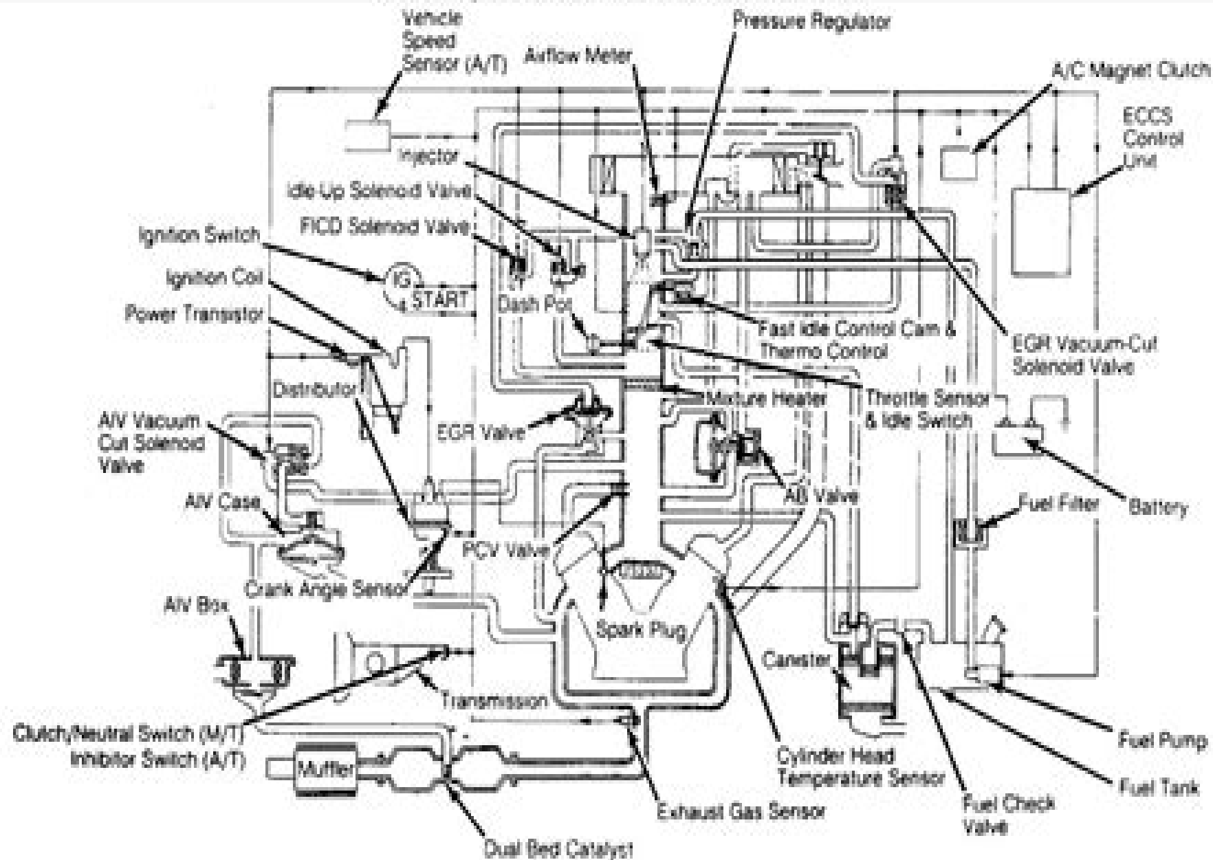
Fig. 3: Vacuum Diagrams (Pathfinder & Pickup With VG30i Engine)
