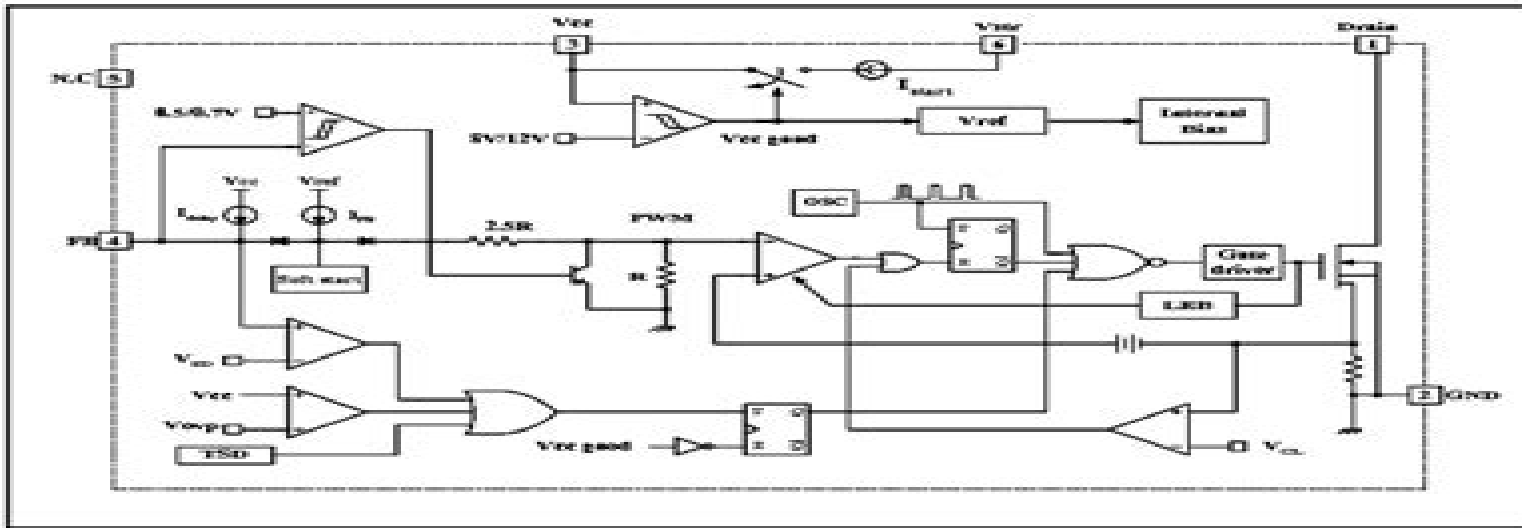
Figure 2. Functional Block Diagram of FSDM0565RB
