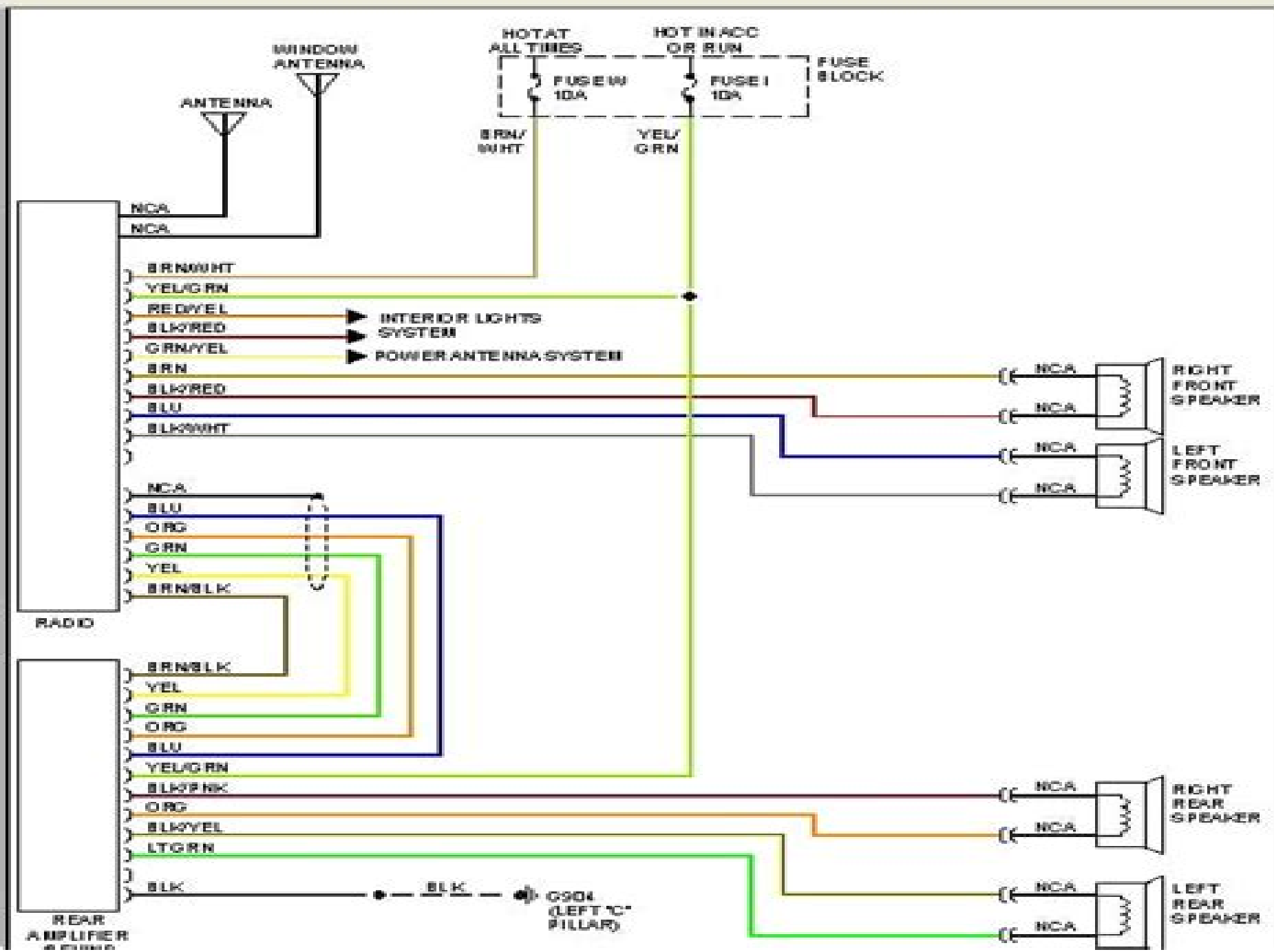
Fig. 14: Radio Circuits, Except Bose
