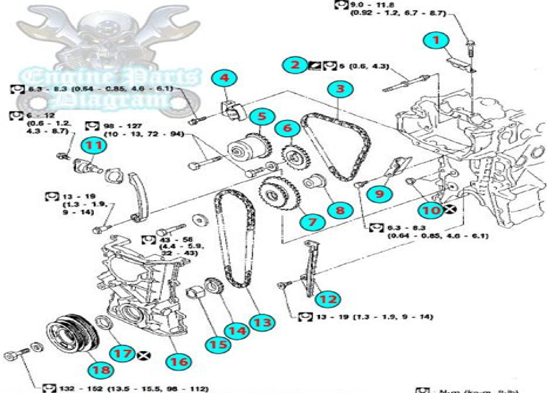
Nissan GA16DE Engine Timing Chain Components
