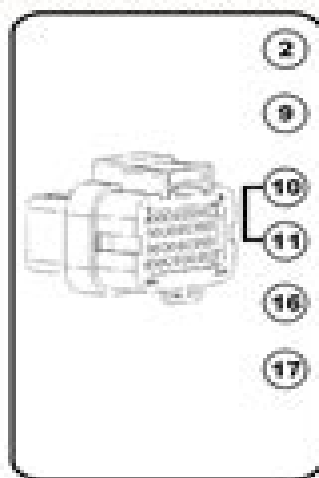
HALTECH ELITE 2500 / 1500 ECU 34 PIN ECU CONNECTOR (A)
