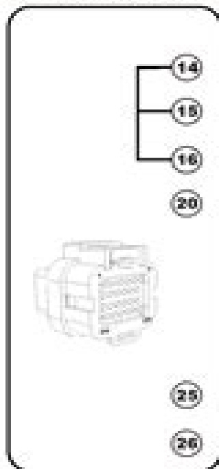
HALTECH ELITE 2500 / 1500 ECU 26 PIN ECU CONNECTOR (B)
