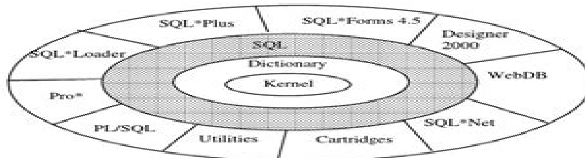
Figure 1: Basic architecture of Oracle
