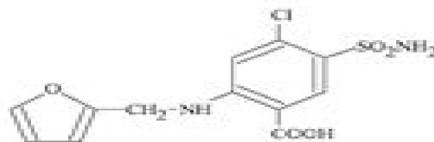
Furosemide
