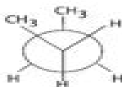
n-Butane
