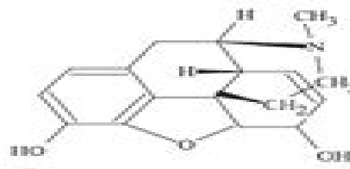
Morphine
