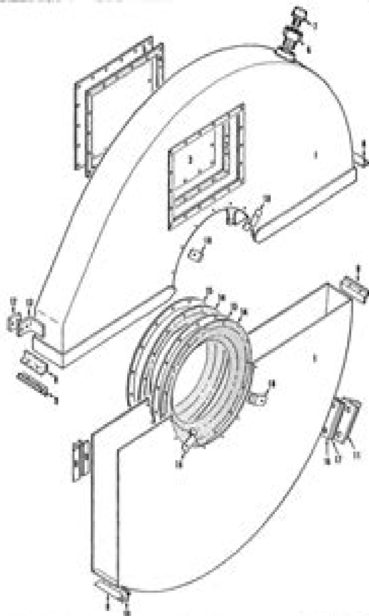
FRONT VIEW OF GEAR CASE
