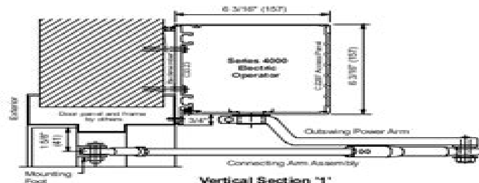
Vertical Section "1"
