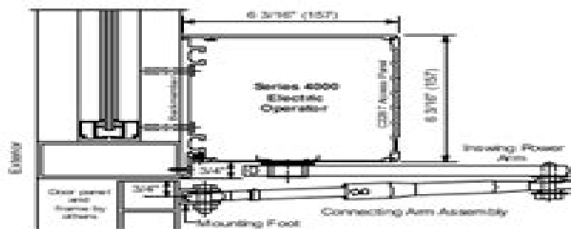
Vertical Section "2"
