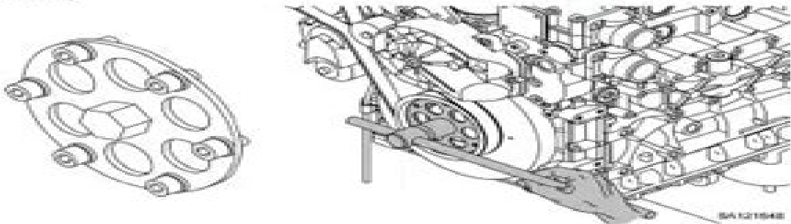
Special tool no. 30a — Mounting the belt pulley crankshaft
