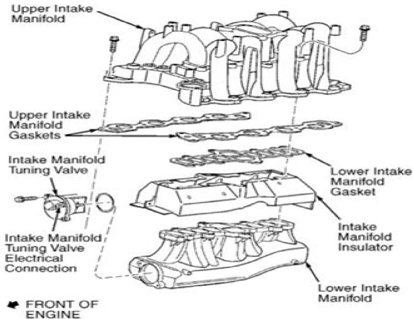
Fig. 2: Exploded View Of Upper & Lower Intake Manifold Courtesy of FORD MOTOR CO.
