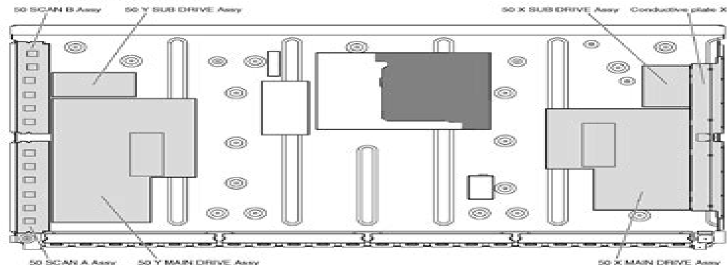
Fig.1 High Voltage Generating Point (Rear view)
