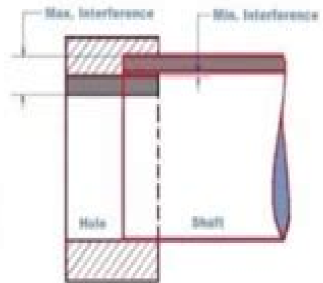
C) Interference Fit
