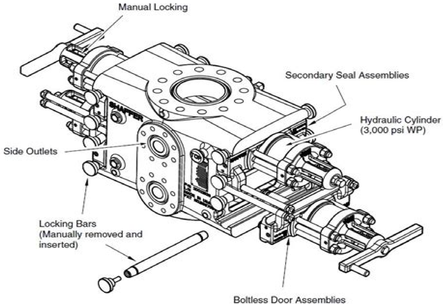
Figure 2-1. LXT Double Blowout Preventer
