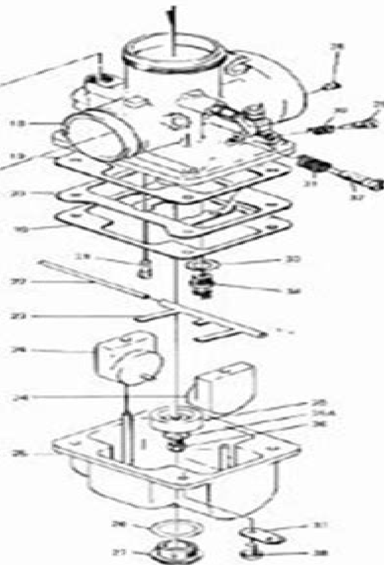
Exploded view of a SPIGOT MOUNT TYPE MIKUNI CARBURETOR
