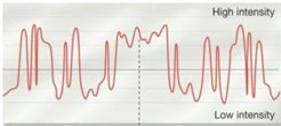
Magnetometer record showing symmetrical magnetic field across ridge
