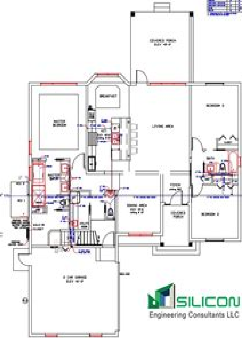
GROUND FLOOR PLAN (DRAINAGE & WATER SUPPLY) TOP & 1/2"
