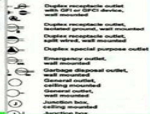
Outlet symbols
