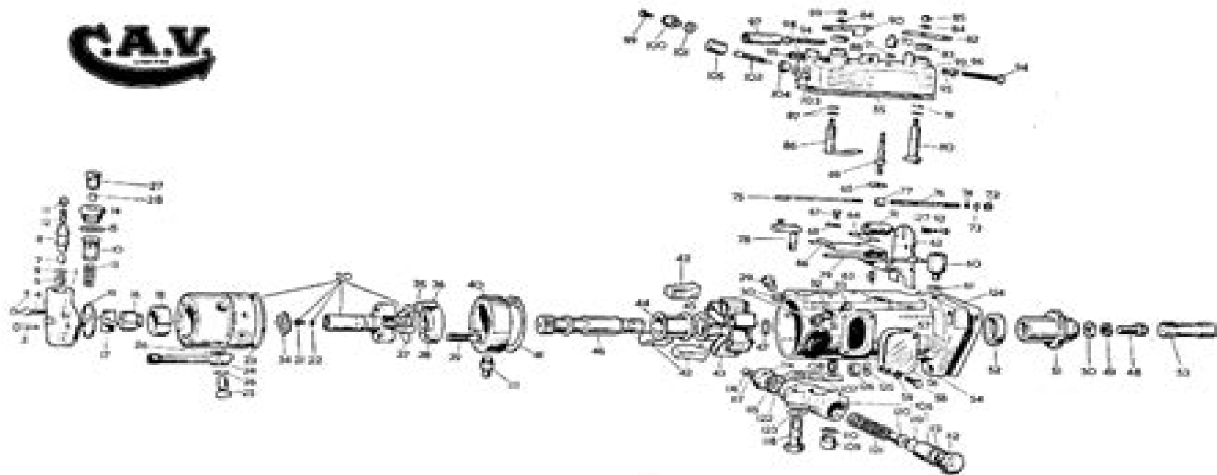
Mechanically Governed CAV DPA pump
