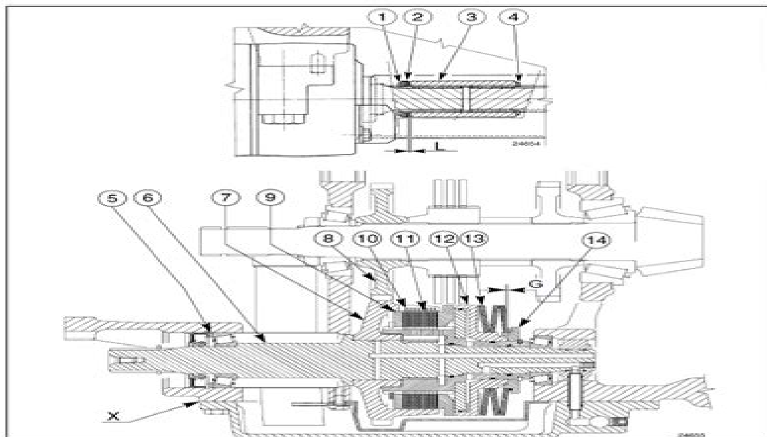
FWD Electro-Hydraulic Clutch Sectional Views
