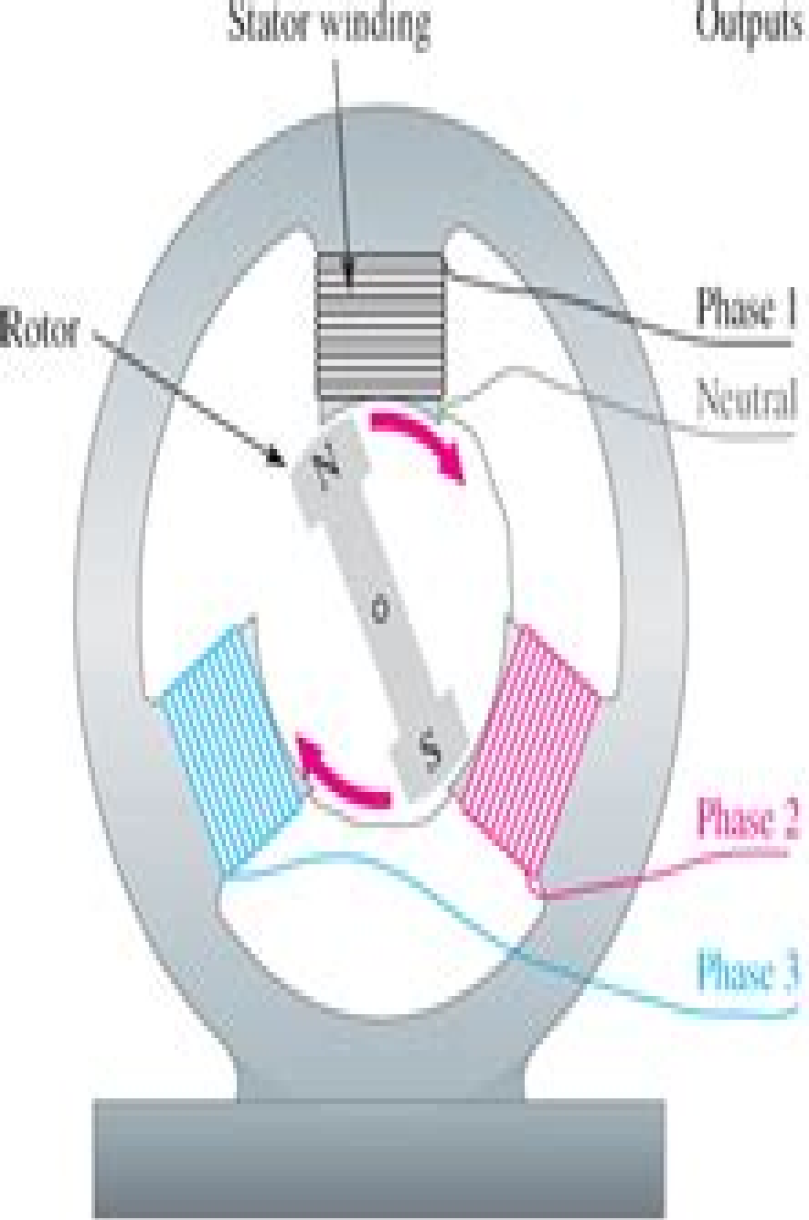
(a) Three-phase rotating-field generator
