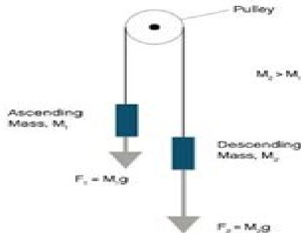
Figure 4: Free Body Diagram: 2 objects with mass hanging on a pulley by string.
