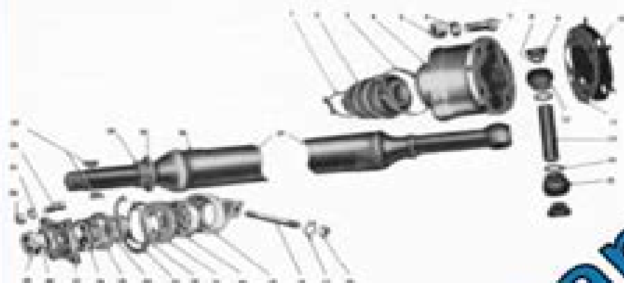
Fig. 515 Front propeller shaft and water pump used in series
