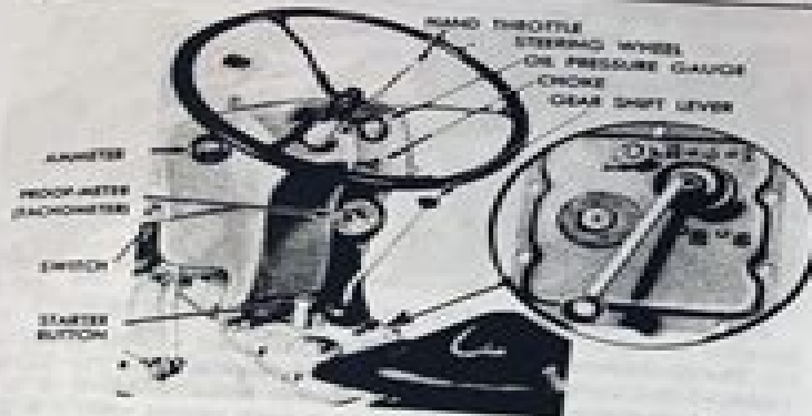
Fig. 5—Operator's Controls
