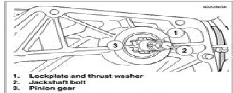
Figure 5-6. Lockplate on Jackshaft Bolt
