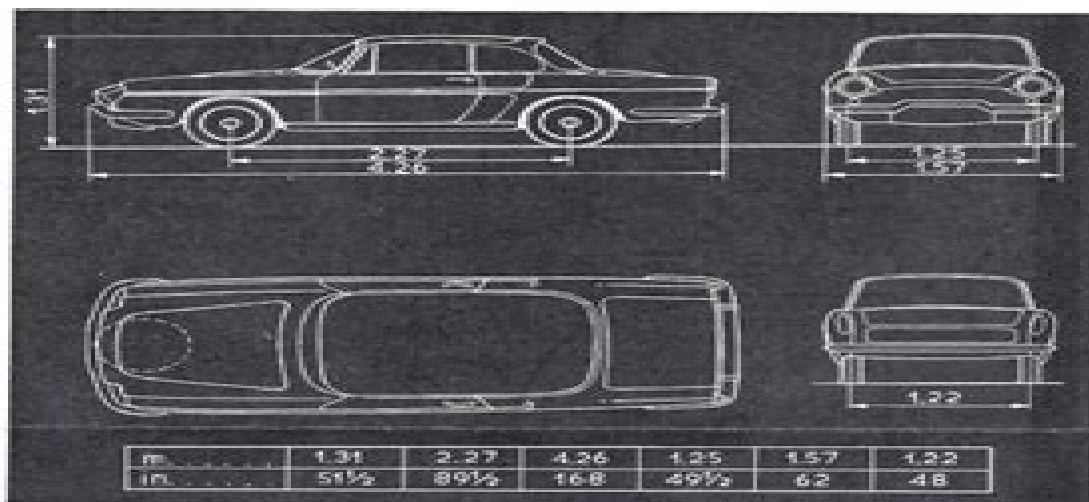
Dimensioned views, showing measurements in English and Metric equivalents
