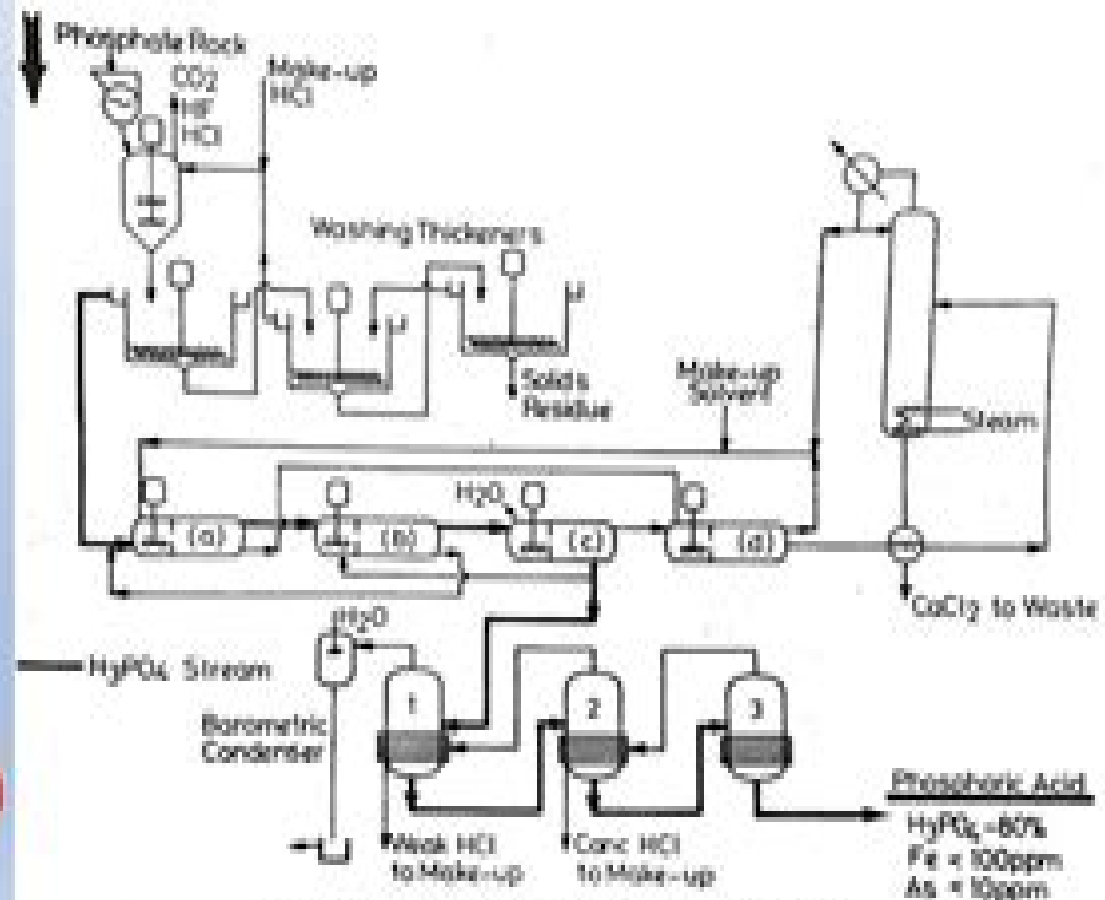
Fig. BP-3. Production of phosphoric acid by HCl leaching.
