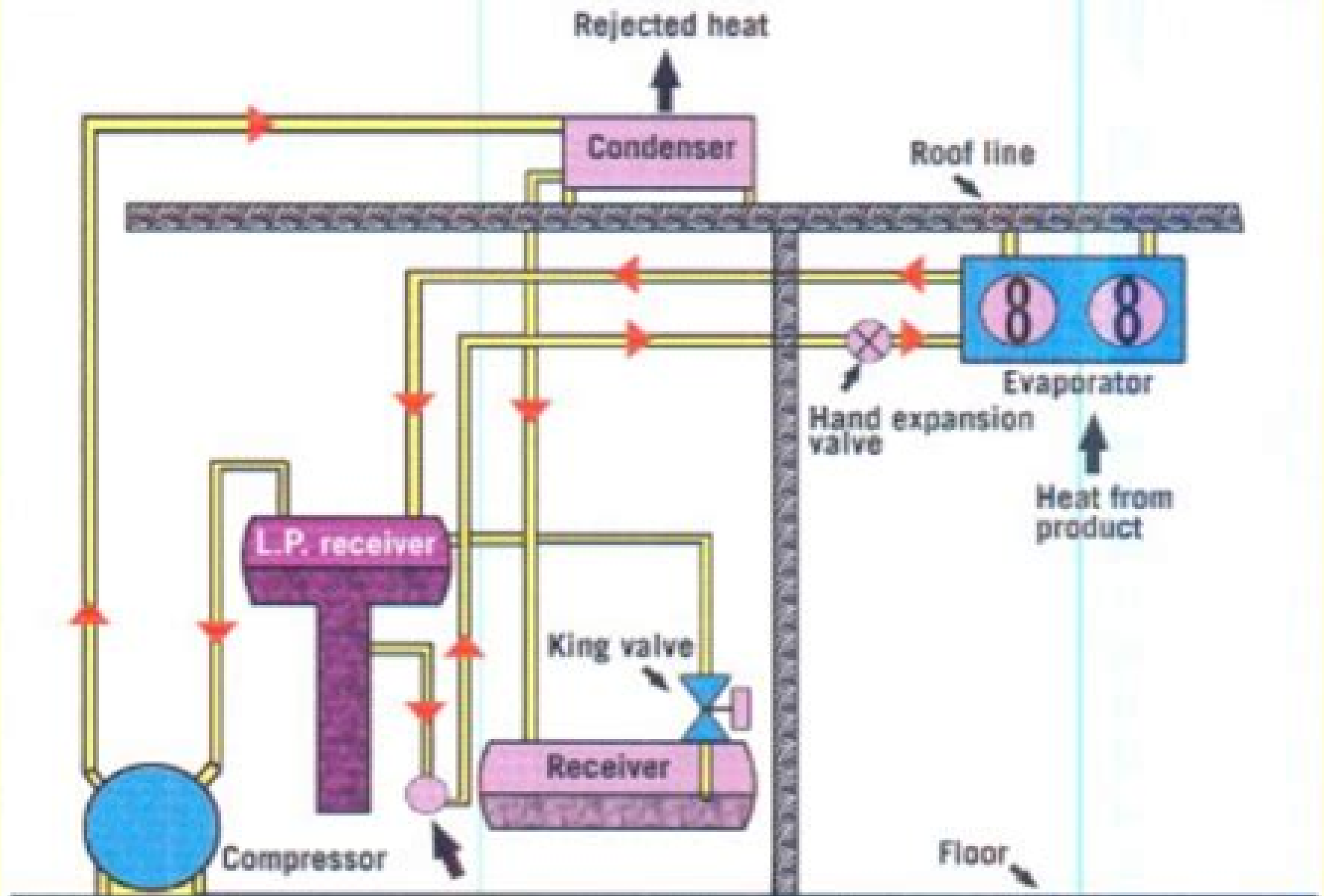
Liquid pump recirculation system
