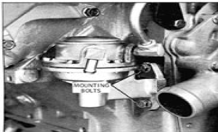
Fig. 3-134 Fuel Pump Mounting
