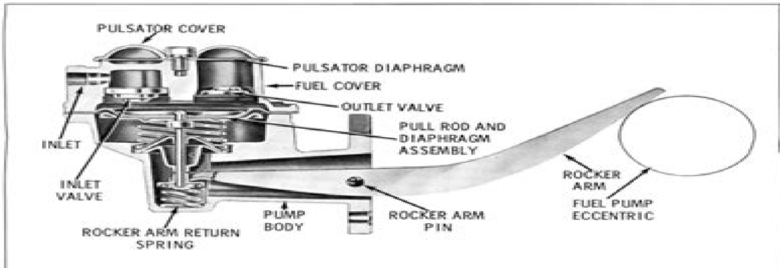
Fig. 3-133 Fuel Pump Assembly
