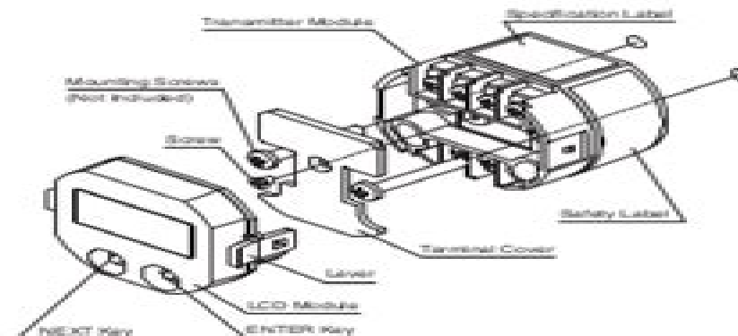
Figure 1. FRC0 exploded view and component identification
