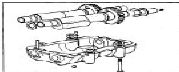
Fig. 37 - Counterbalance weights assembly components.
