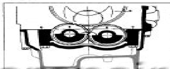
Fig. 38 - Counterbalance weights assembly.
