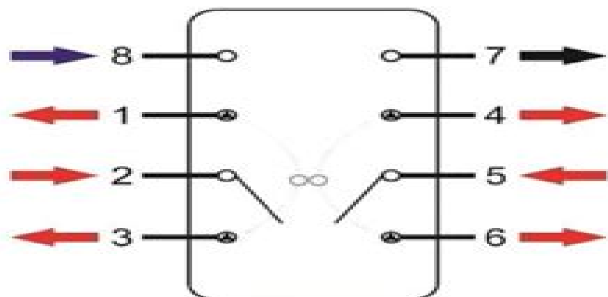
CIRCUIT DIAGRAM
