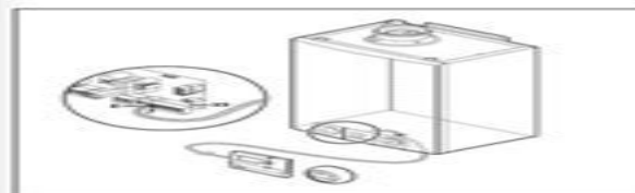
Connecting Open Thermo room controls (e.g. the Baxi Thermo TC or TC2). Mount the control in a convenient room (usually the living room). Connect the two-wire interface cables to connections 7 and 8 of the J2 terminal strip. When using the Control TC 2 it is possible to add the outdoor sensor to provide weather compensation with room adjustment. Connect the outside sensor to connections 1 and 2 of the J2 terminal strip.
