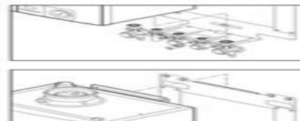
3. Fit flow washers on HTG Valves. Suspend the boiler on mounting plate.
