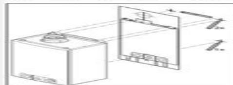
1. Using the template determine and mark the position of the three mounting holes, making sure the plate is absolutely level.
