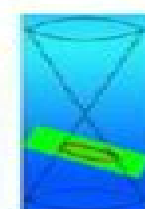
Ellipse
