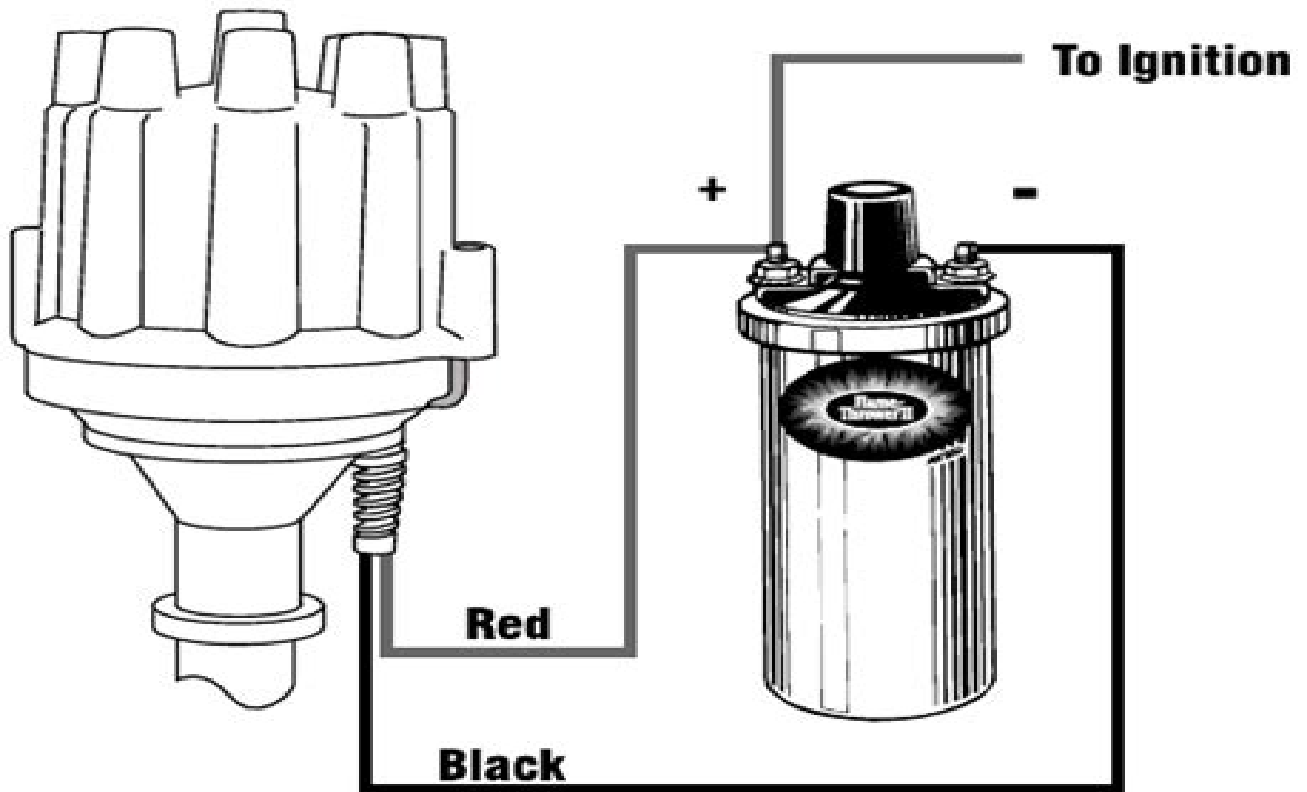
FIGURE 3 (WITHOUT EXTERNAL RESISTOR)
